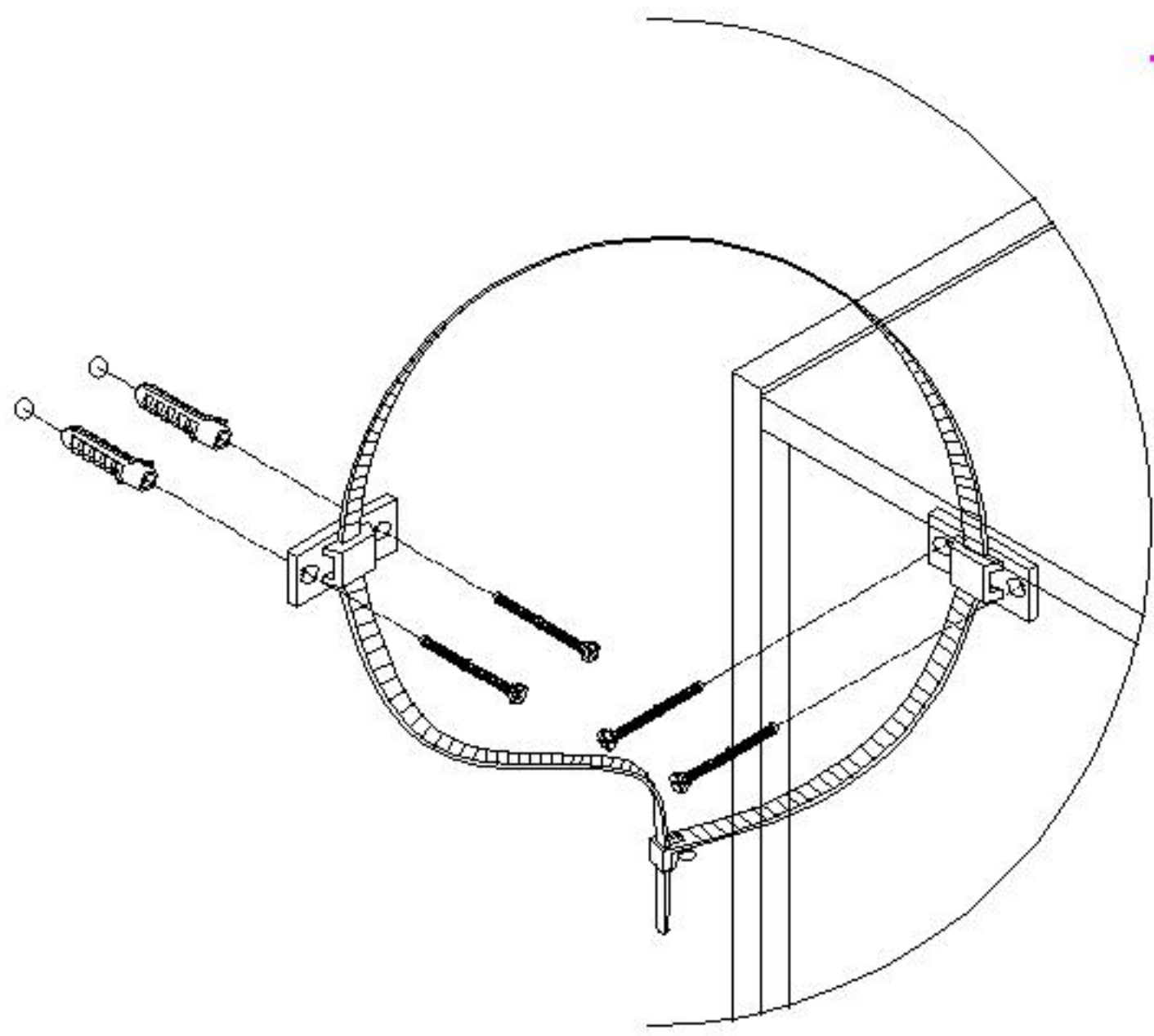
N处放大图 Enlarged view at N
