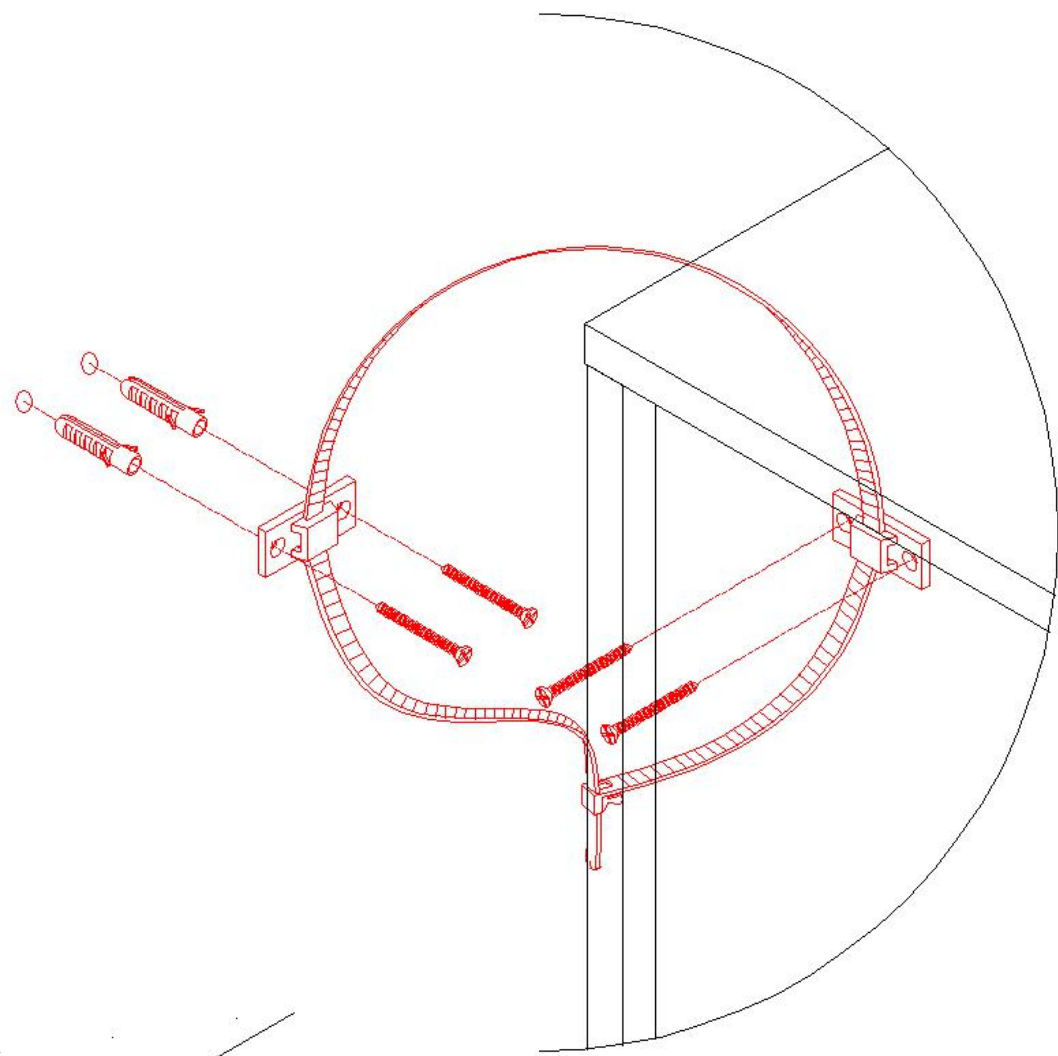
T处放大图 Enlarged view at T
